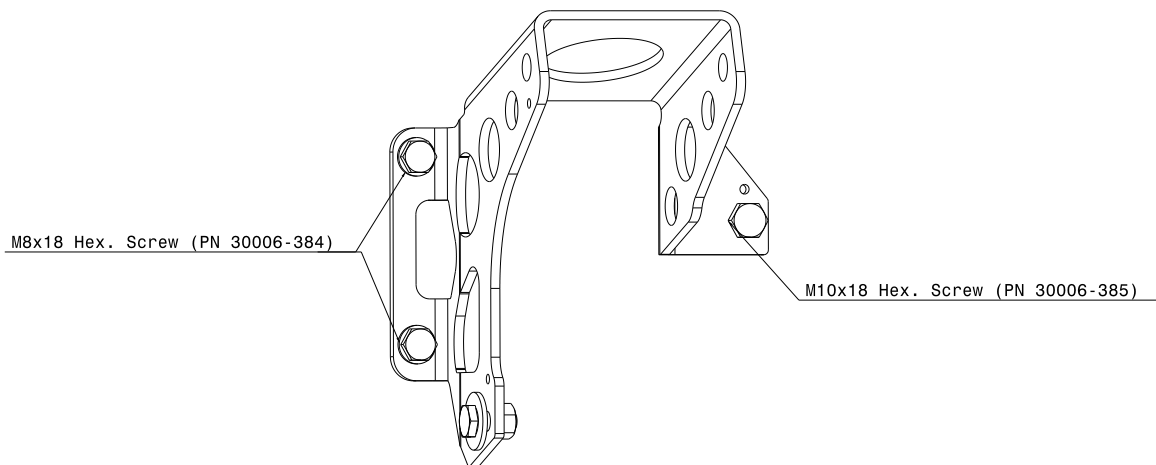
Figure 4-12 : Isometric view Mounting Frame 70A 915iS
