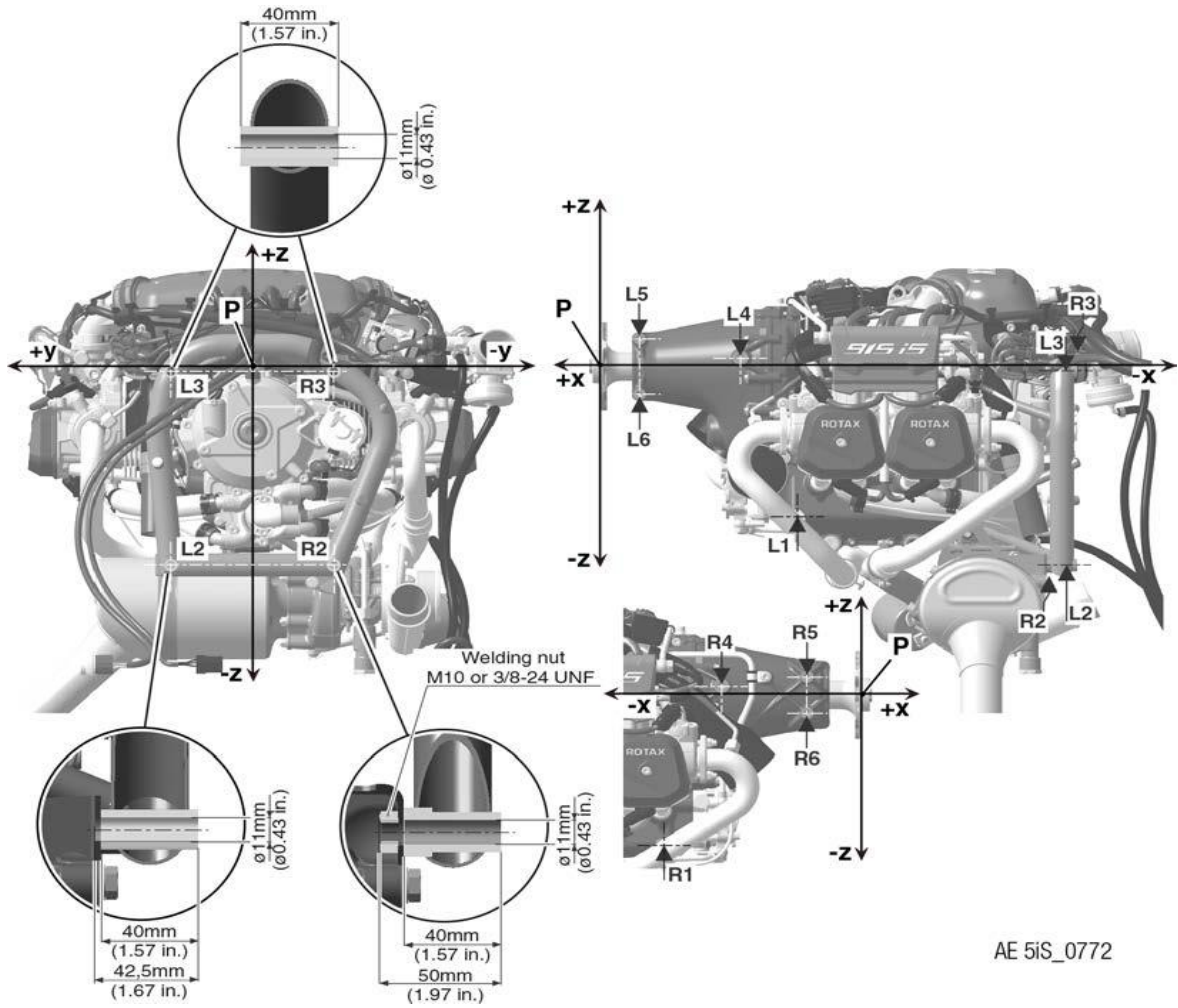
Figure 4-16: 915iS Attachment points
