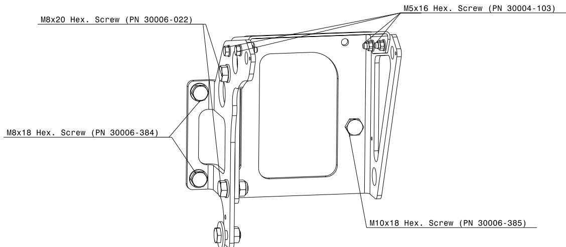
Figure 4-14 : Isometric view Side Frames 150A 915iS
