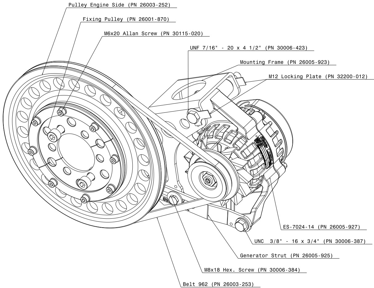
Figure 4-11 : Isometric view 70A 915iS
