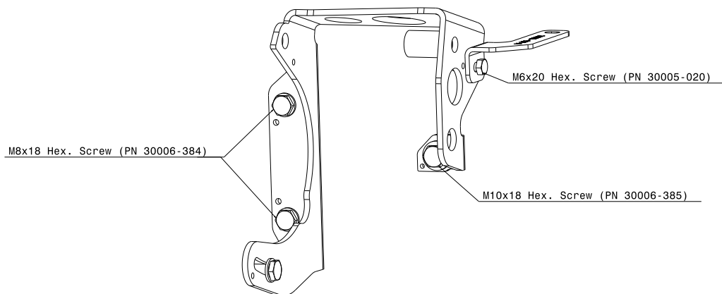
Figure 4-10 : Isometric view Mounting Frame 20A 915iS
