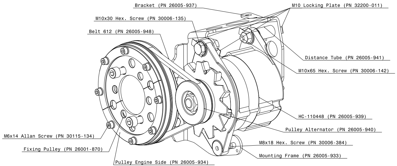
Figure 4-9 : Isometric view 20A 915iS
