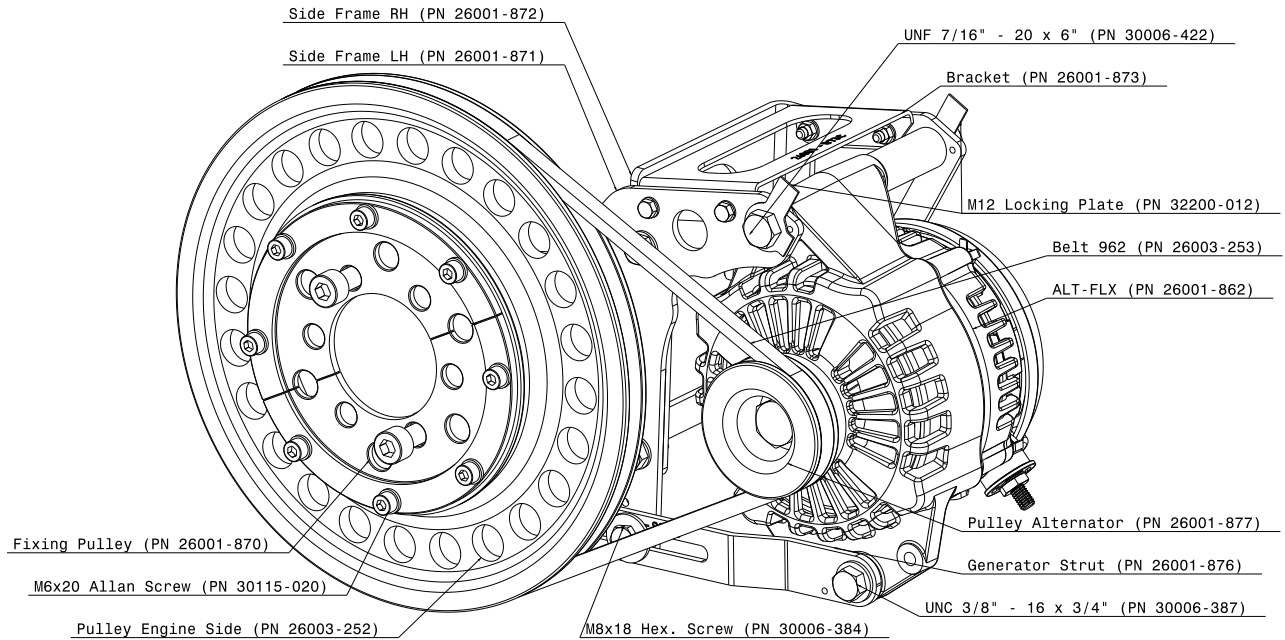
Figure 4-13 : Isometric view 150A 915iS
