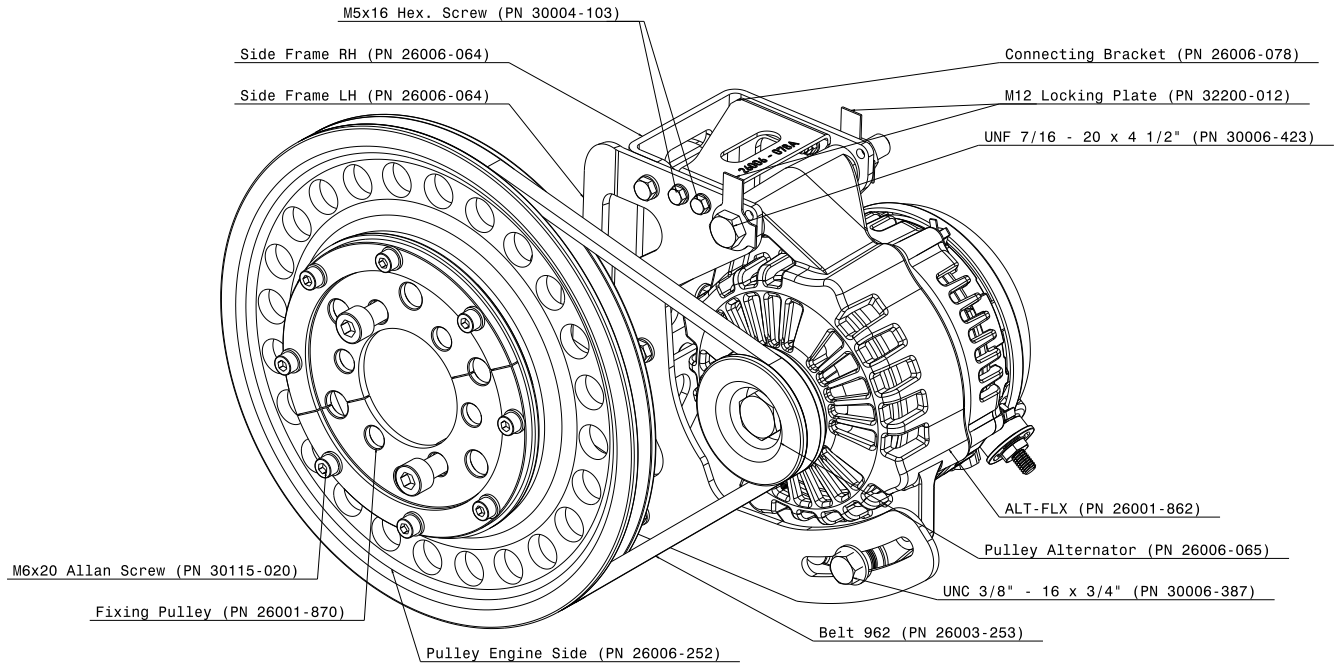
Figure 4-7 : Isometric view 150A 912iS
